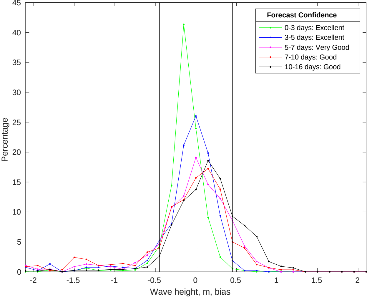
NDBC 41013 vs GFS Waves Bias Histogram: 16-Jul-2025
