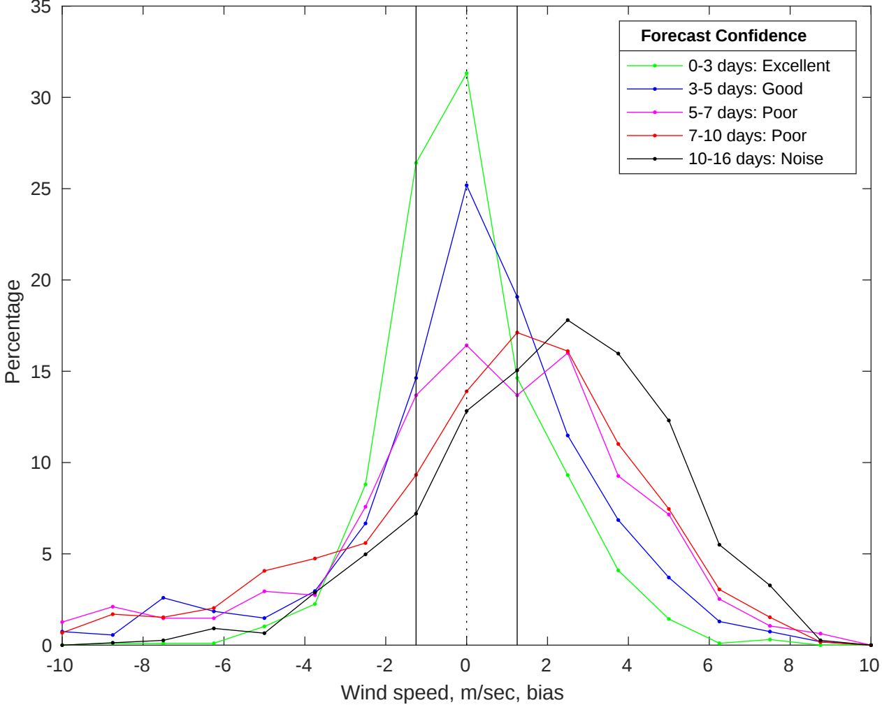
NDBC 41013 vs GFS Winds Bias Histogram: 16-Jul-2025
