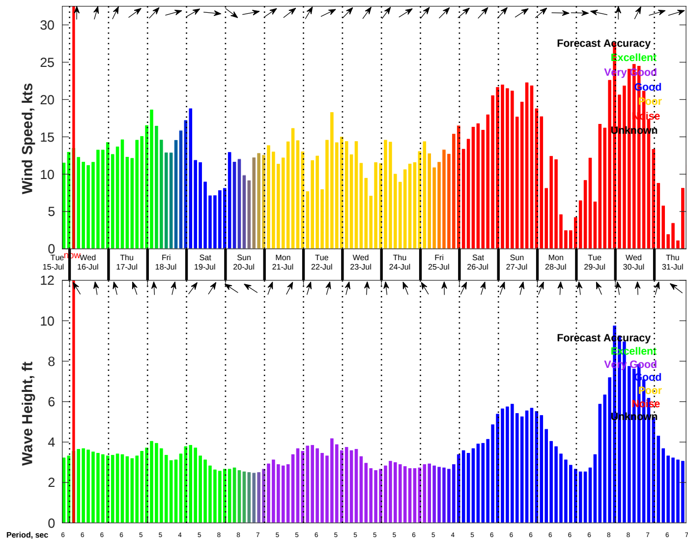
Wind & Wave Forecast for NDBC 41013 from 15-Jul-2025 19:00:00 to 31-Jul-2025 19:00:00
