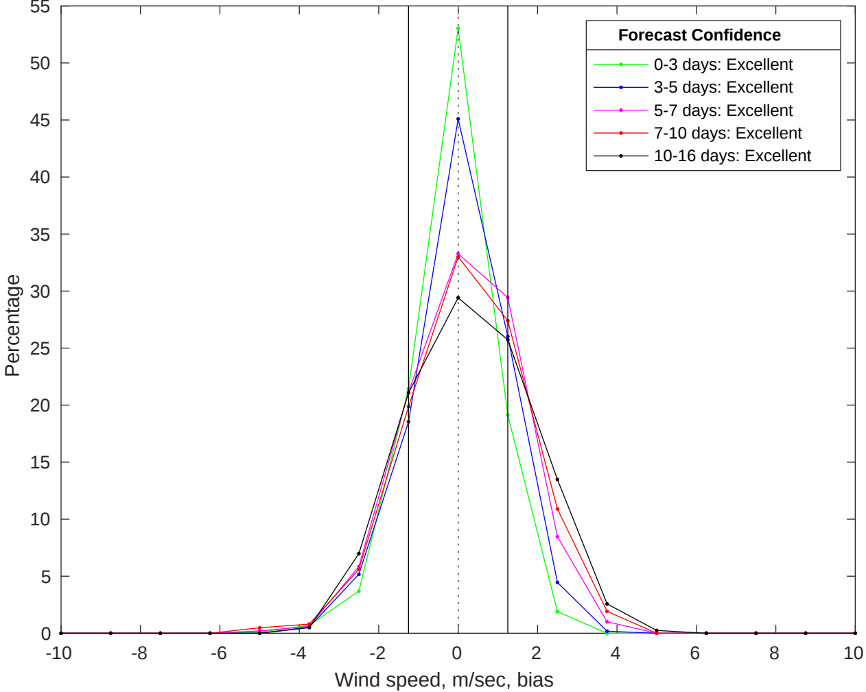
NDBC 41040 vs GFS Winds Bias Histogram: 16-Jul-2025
