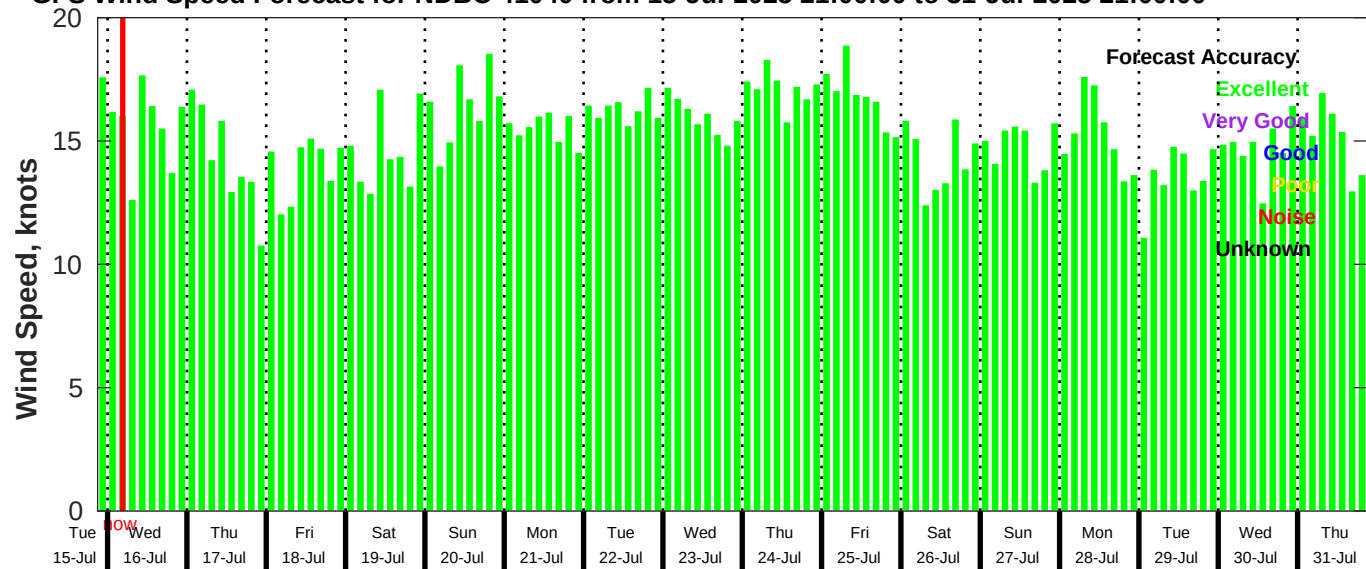
GFS Wind Speed Forecast for NDBC 41040 from 15-Jul-2025 21:00:00 to 31-Jul-2025 21:00:00
