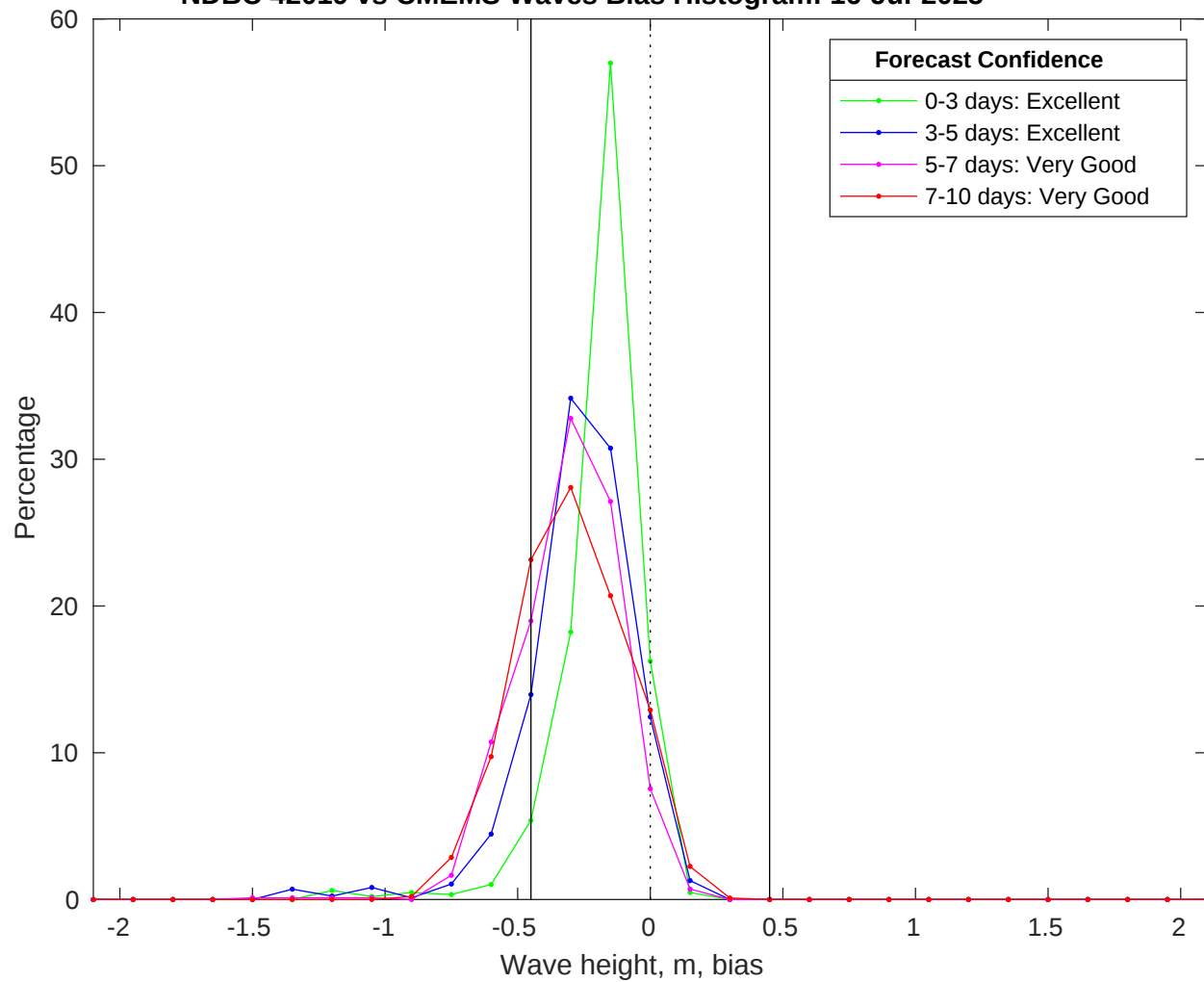
NDBC 42019 vs CMEMS Waves Bias Histogram: 16-Jul-2025
