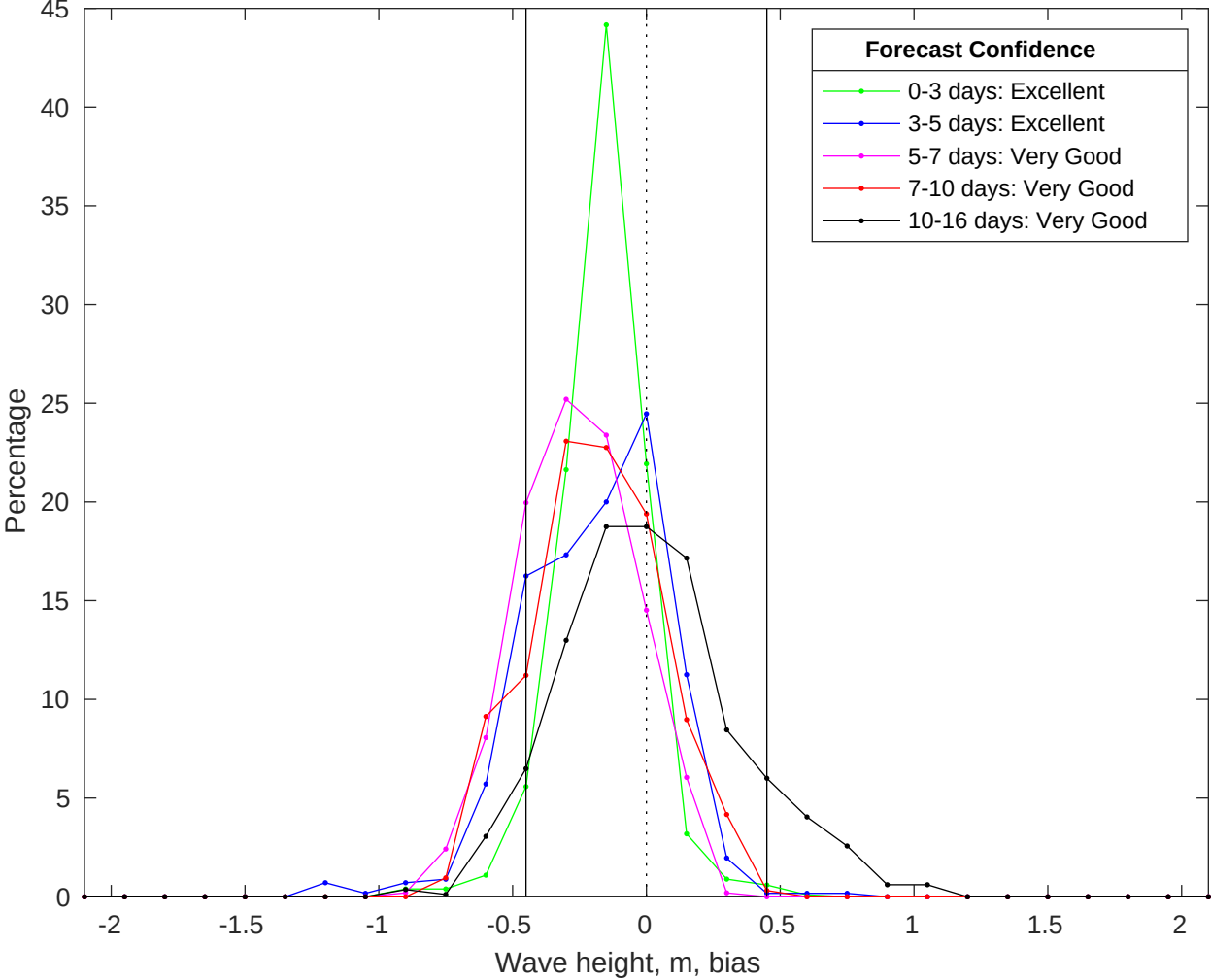
NDBC 42019 vs GFS Waves Bias Histogram: 16-Jul-2025
