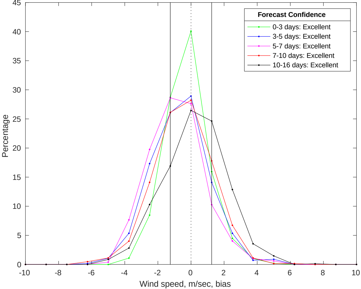
NDBC 42019 vs GFS Winds Bias Histogram: 16-Jul-2025
