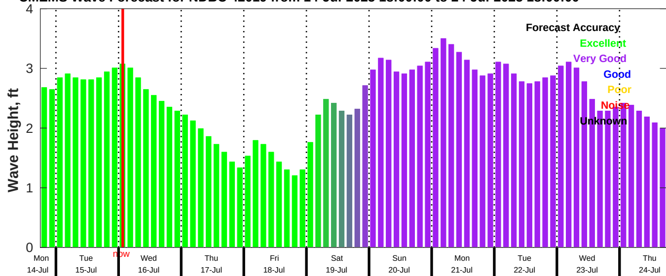
CMEMS Wave Forecast for NDBC 42019 from 14-Jul-2025 18:00:00 to 24-Jul-2025 18:00:00
