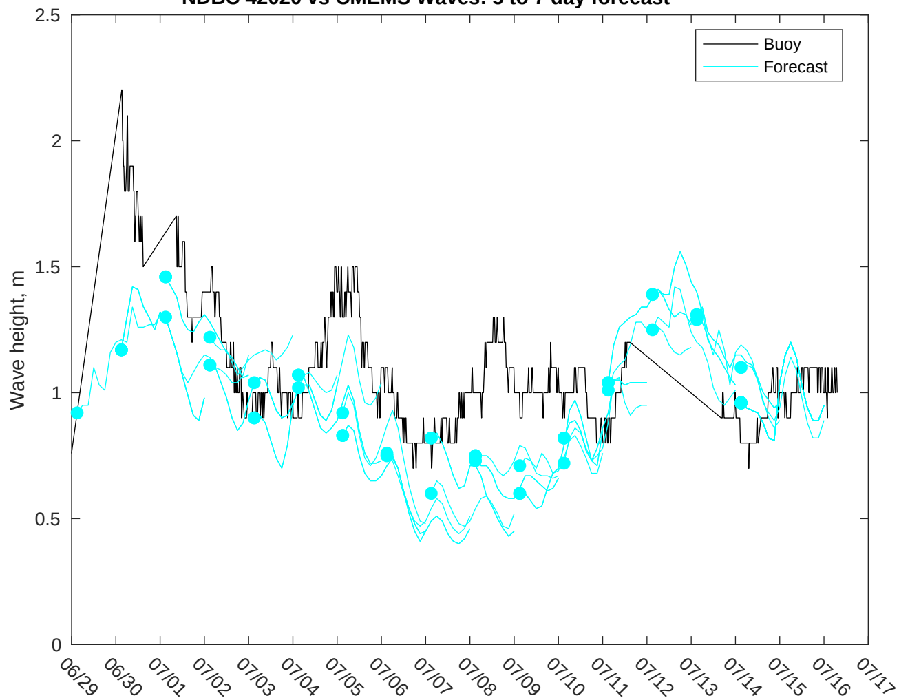
NDBC 42020 vs CMEMS Waves: 5 to 7 day forecast
