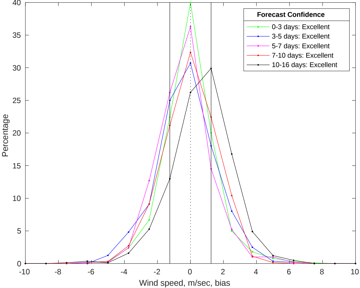
NDBC 42020 vs GFS Winds Bias Histogram: 16-Jul-2025
