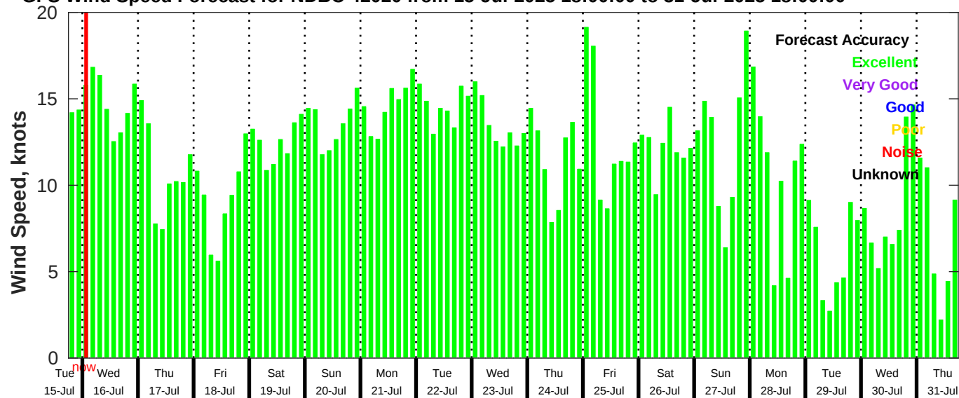
GFS Wind Speed Forecast for NDBC 42020 from 15-Jul-2025 18:00:00 to 31-Jul-2025 18:00:00
