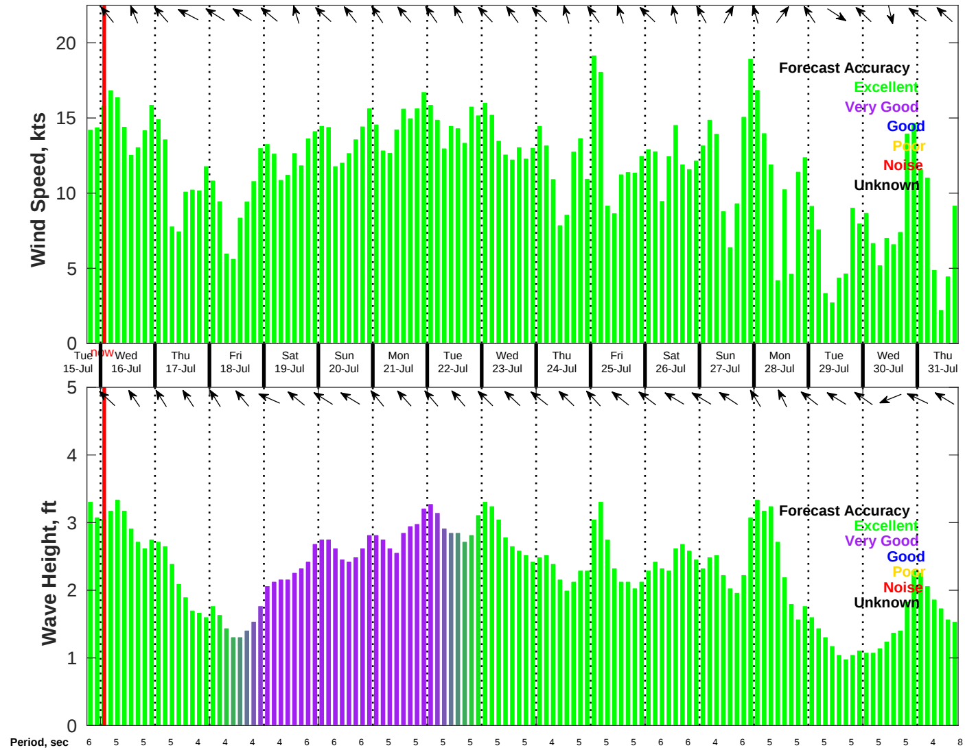
Wind & Wave Forecast for NDBC 42020 from 15-Jul-2025 18:00:00 to 31-Jul-2025 18:00:00
