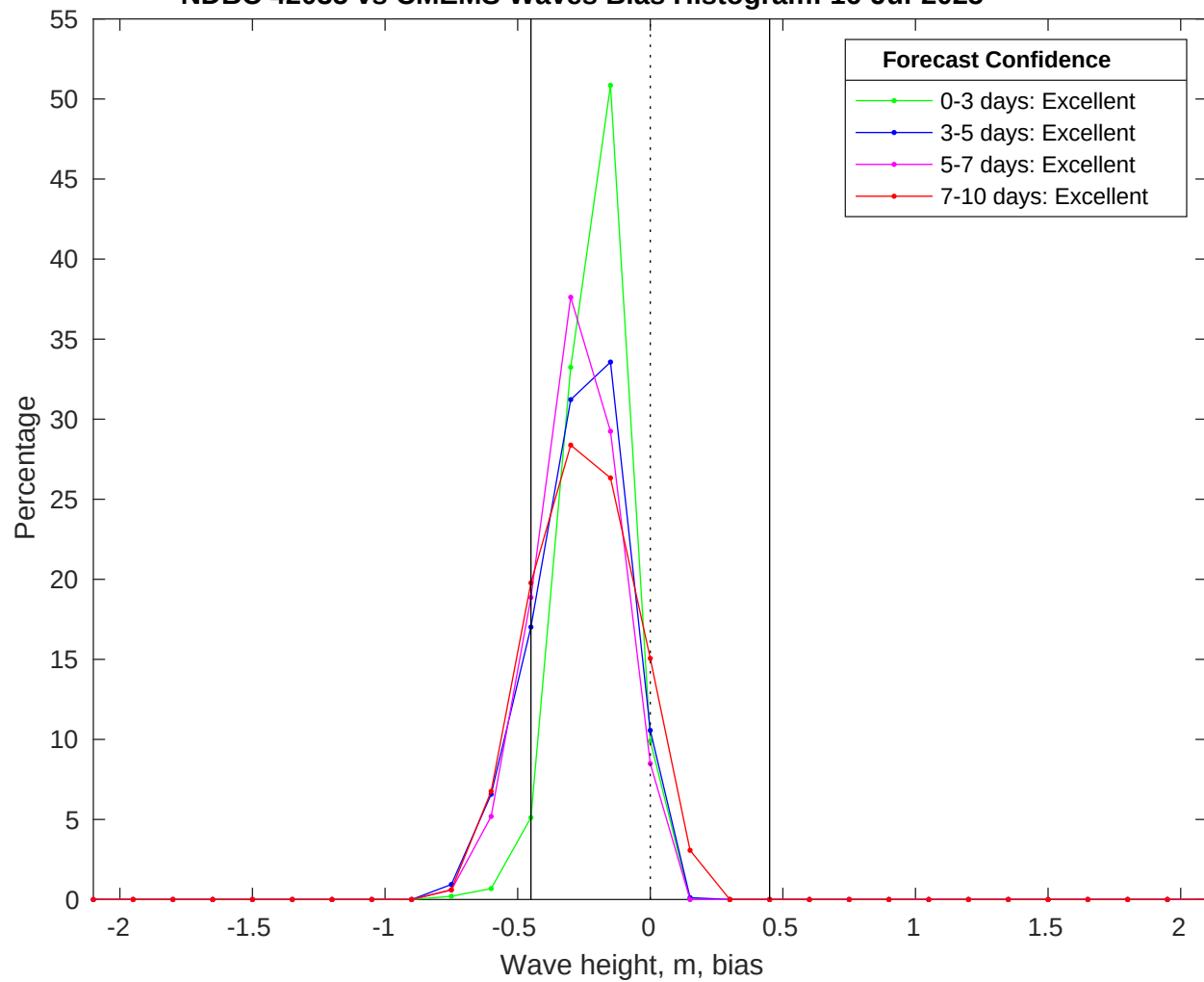
NDBC 42035 vs CMEMS Waves Bias Histogram: 16-Jul-2025
