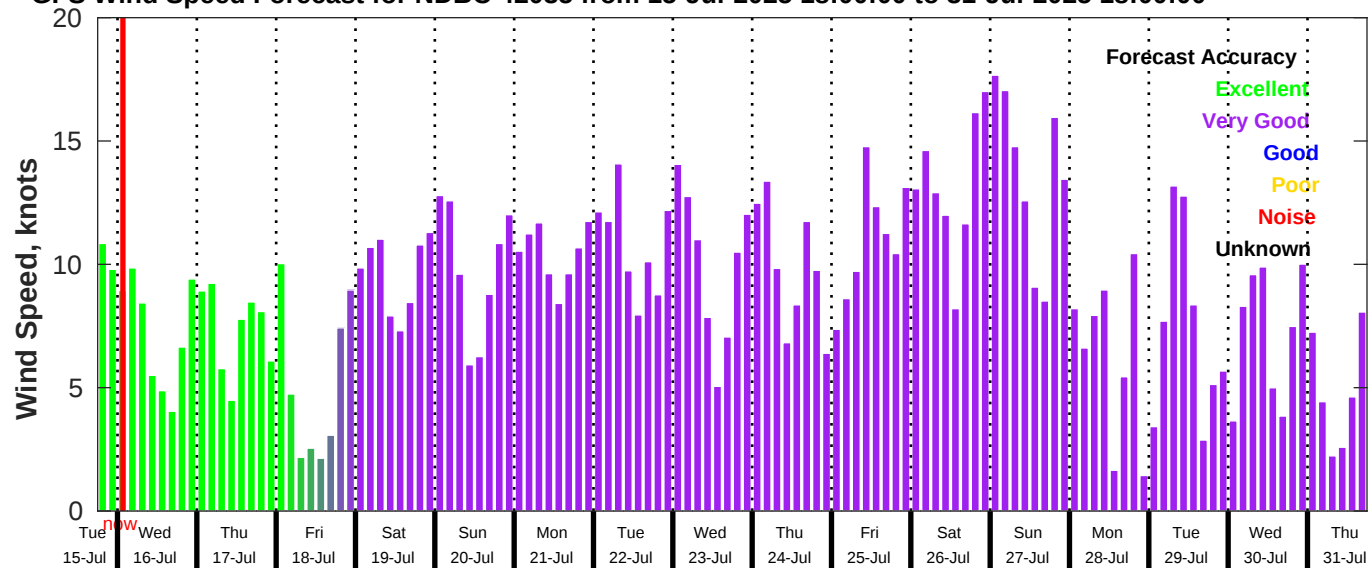
GFS Wind Speed Forecast for NDBC 42035 from 15-Jul-2025 18:00:00 to 31-Jul-2025 18:00:00
