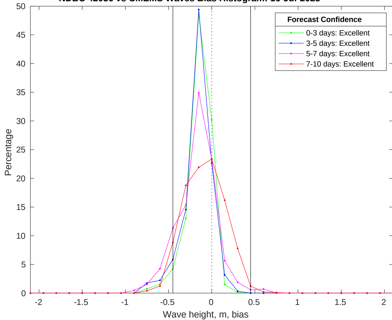
NDBC 42036 vs CMEMS Waves Bias Histogram: 16-Jul-2025
