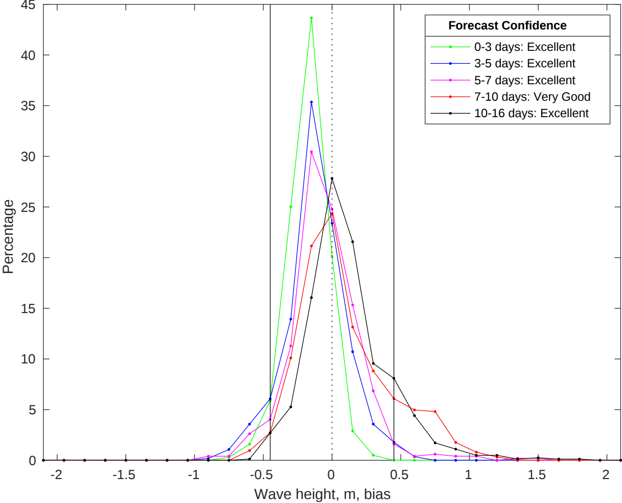
NDBC 42036 vs GFS Waves Bias Histogram: 16-Jul-2025
