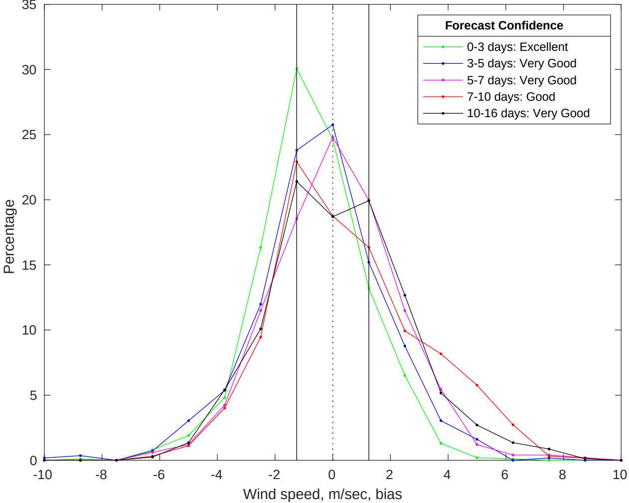
NDBC 42036 vs GFS Winds Bias Histogram: 16-Jul-2025
