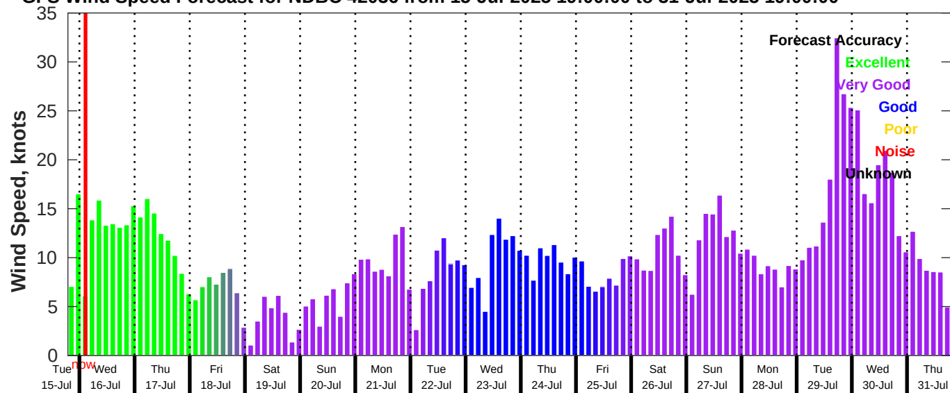
GFS Wind Speed Forecast for NDBC 42036 from 15-Jul-2025 19:00:00 to 31-Jul-2025 19:00:00
