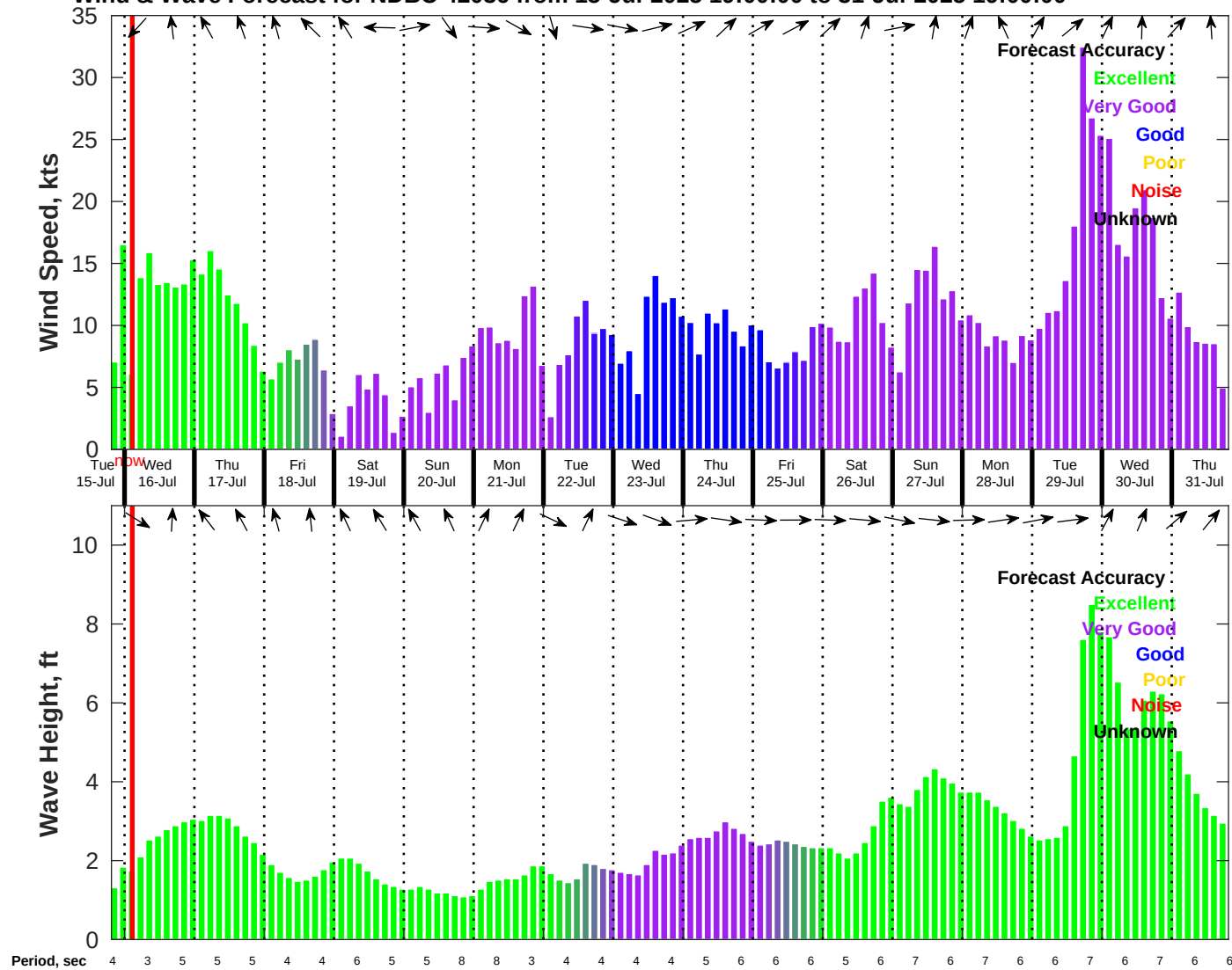
Wind & Wave Forecast for NDBC 42036 from 15-Jul-2025 19:00:00 to 31-Jul-2025 19:00:00
