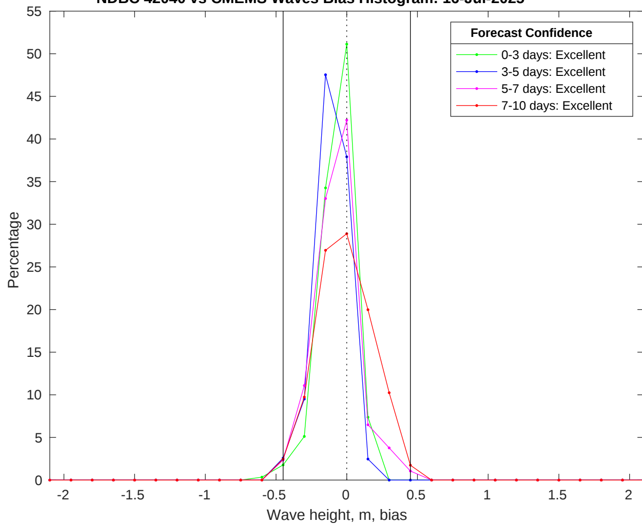
NDBC 42040 vs CMEMS Waves Bias Histogram: 16-Jul-2025
