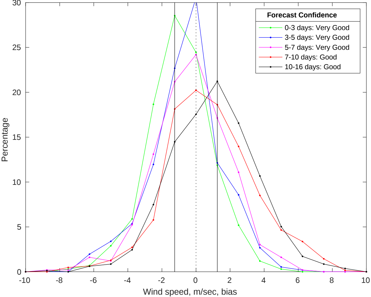
NDBC 42040 vs GFS Winds Bias Histogram: 16-Jul-2025
