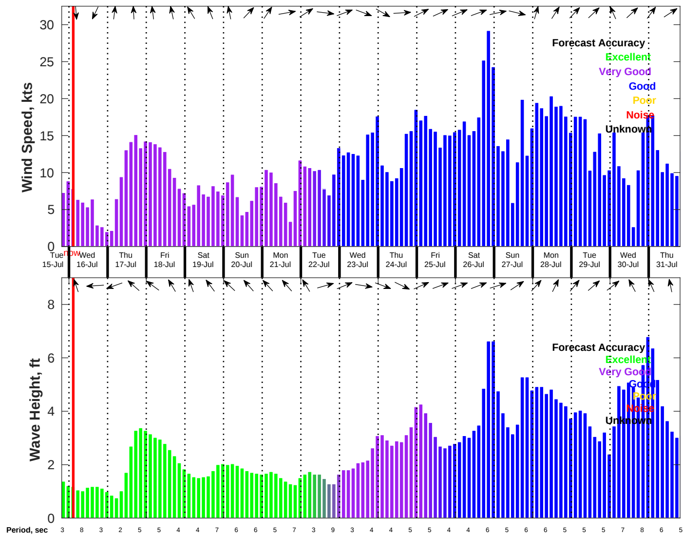
Wind & Wave Forecast for NDBC 42040 from 15-Jul-2025 19:00:00 to 31-Jul-2025 19:00:00
