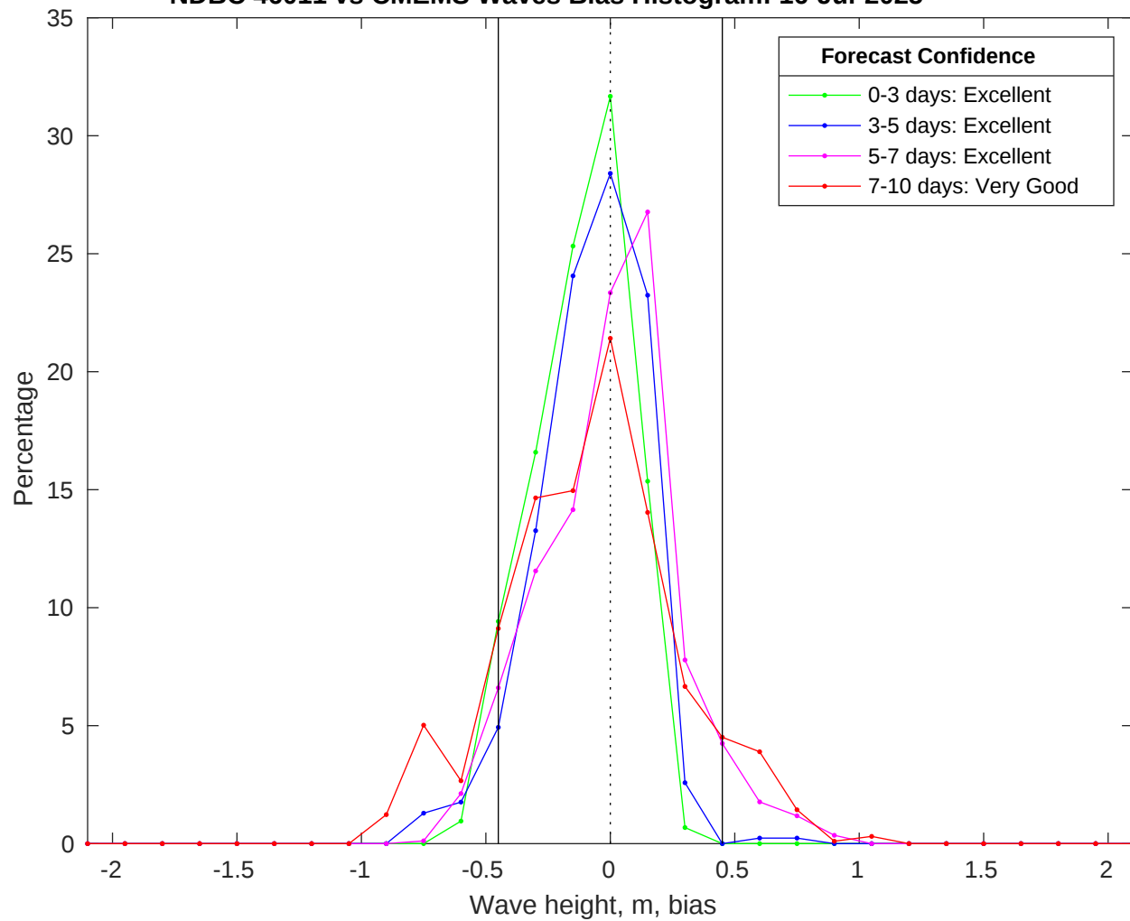
NDBC 46011 vs CMEMS Waves Bias Histogram: 16-Jul-2025
