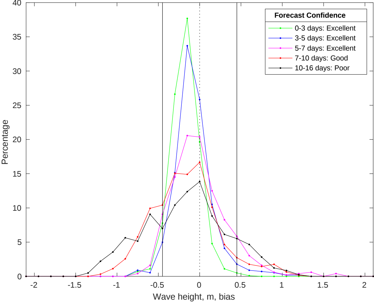
NDBC 46011 vs GFS Waves Bias Histogram: 16-Jul-2025
