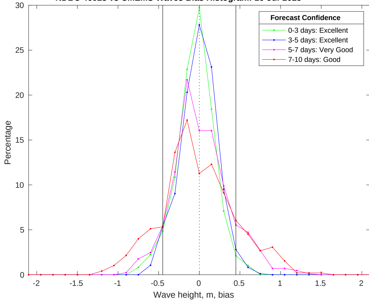
NDBC 46028 vs CMEMS Waves Bias Histogram: 16-Jul-2025
