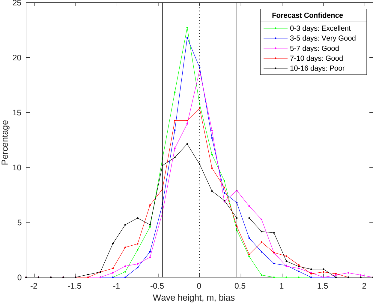
NDBC 46028 vs GFS Waves Bias Histogram: 16-Jul-2025
