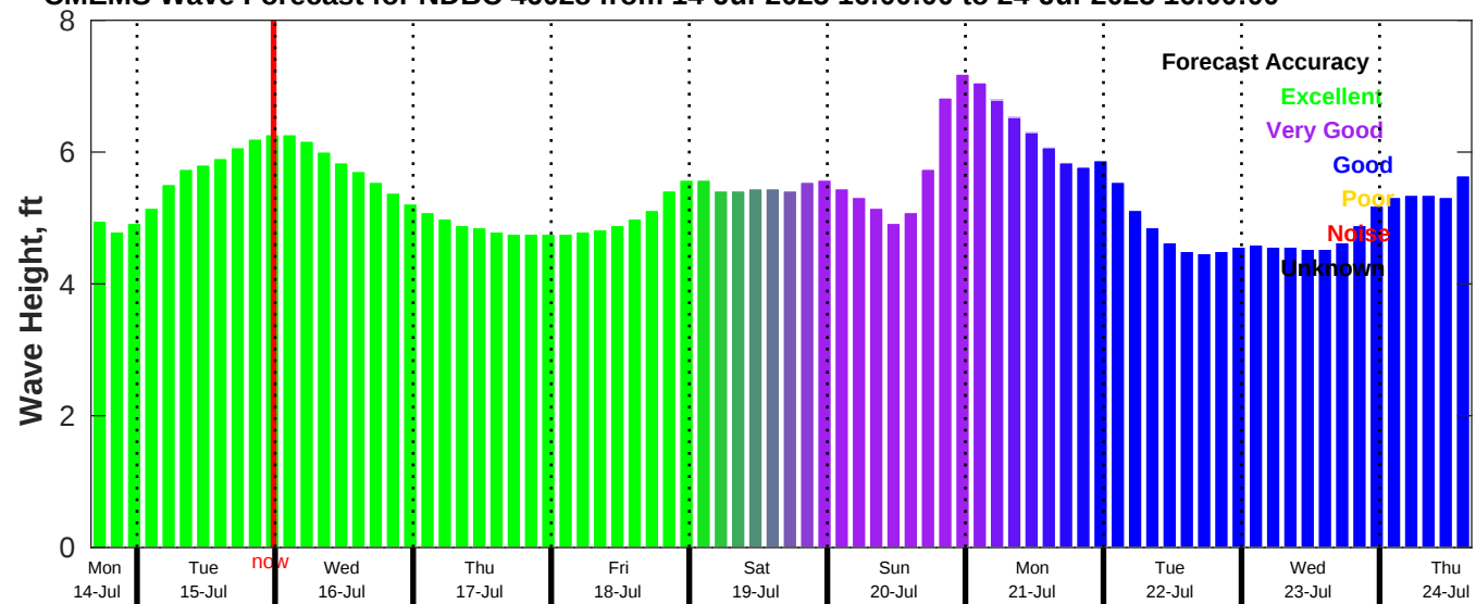
CMEMS Wave Forecast for NDBC 46028 from 14-Jul-2025 16:00:00 to 24-Jul-2025 16:00:00
