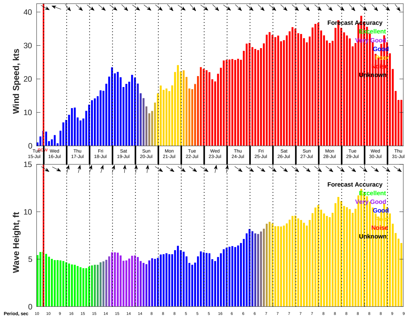
Wind & Wave Forecast for NDBC 46028 from 15-Jul-2025 16:00:00 to 31-Jul-2025 16:00:00
