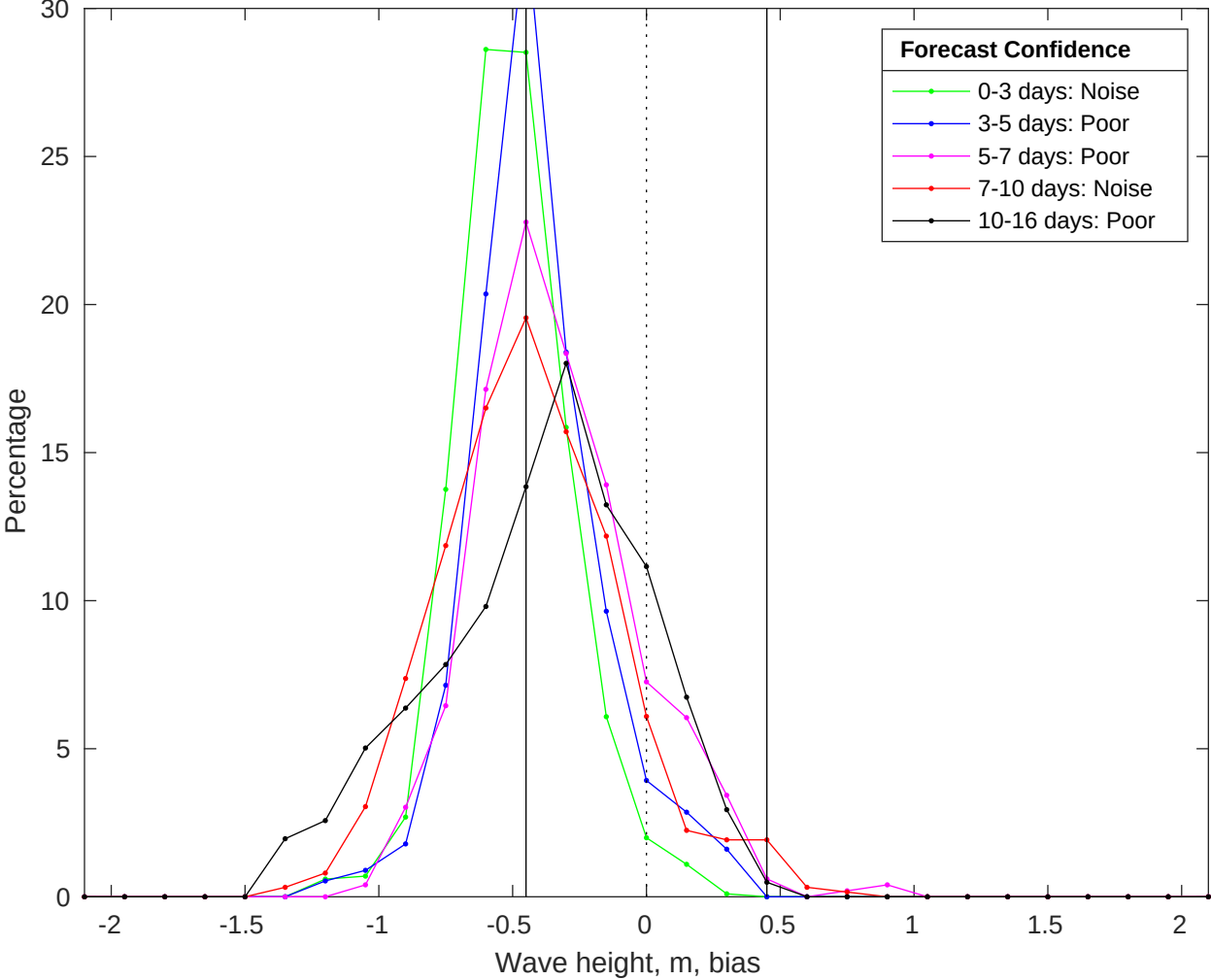
NDBC 46054 vs GFS Waves Bias Histogram: 16-Jul-2025
