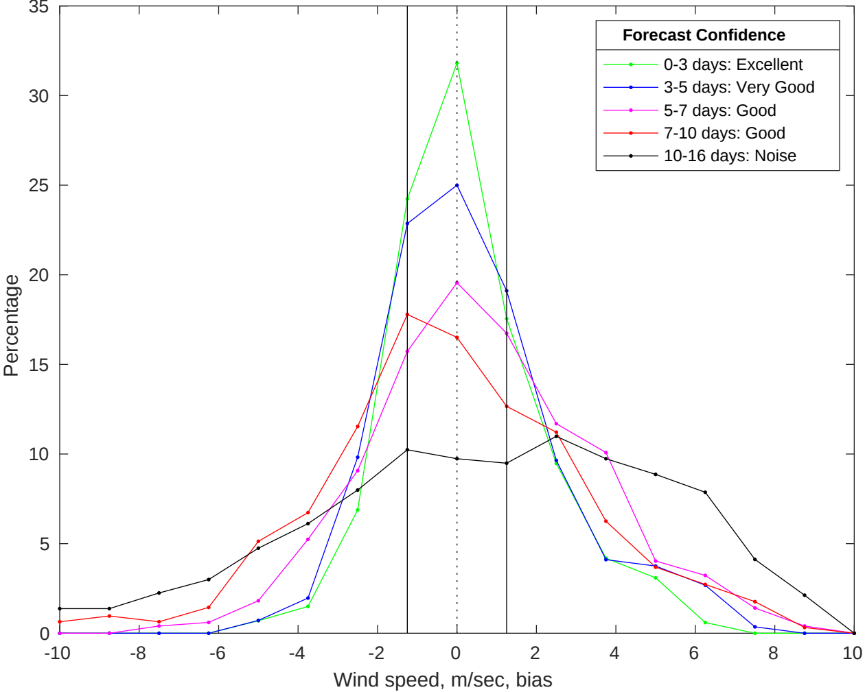
NDBC 46054 vs GFS Winds Bias Histogram: 16-Jul-2025
