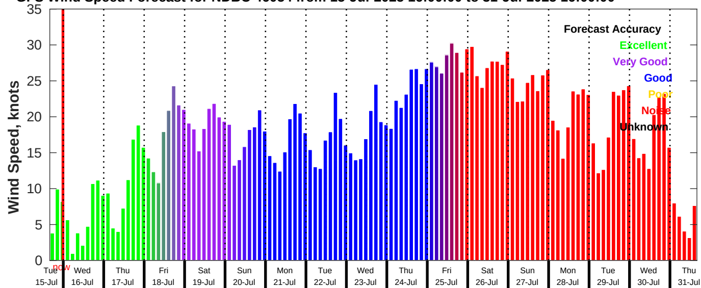
GFS Wind Speed Forecast for NDBC 46054 from 15-Jul-2025 16:00:00 to 31-Jul-2025 16:00:00
