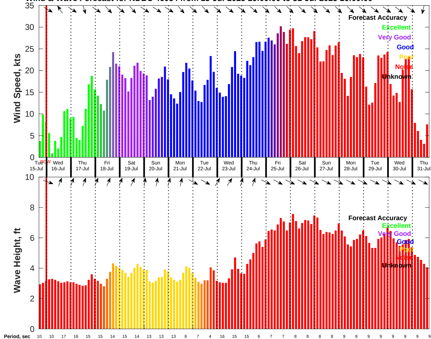
Wind & Wave Forecast for NDBC 46054 from 15-Jul-2025 16:00:00 to 31-Jul-2025 16:00:00
