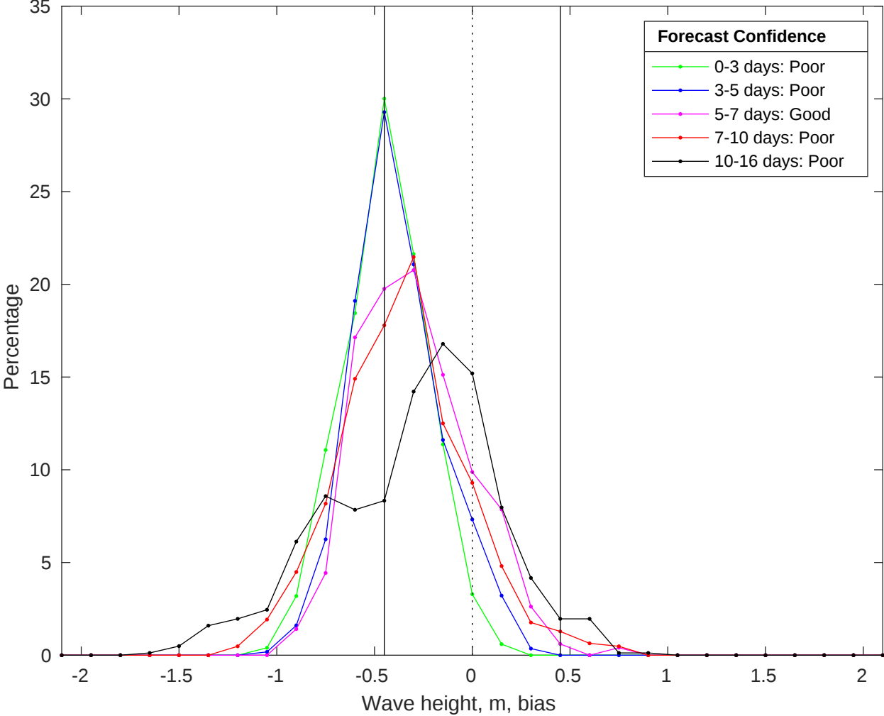
NDBC 46069 vs GFS Waves Bias Histogram: 16-Jul-2025
