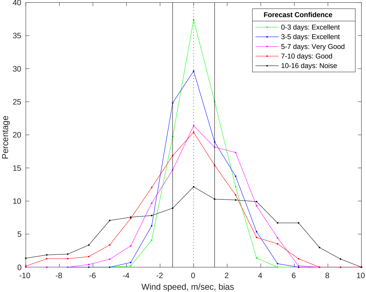
NDBC 46069 vs GFS Winds Bias Histogram: 16-Jul-2025
