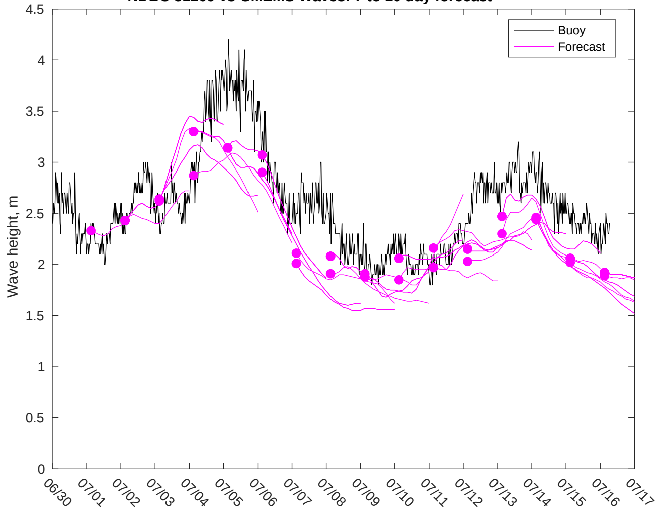
NDBC 51209 vs CMEMS Waves: 7 to 10 day forecast
