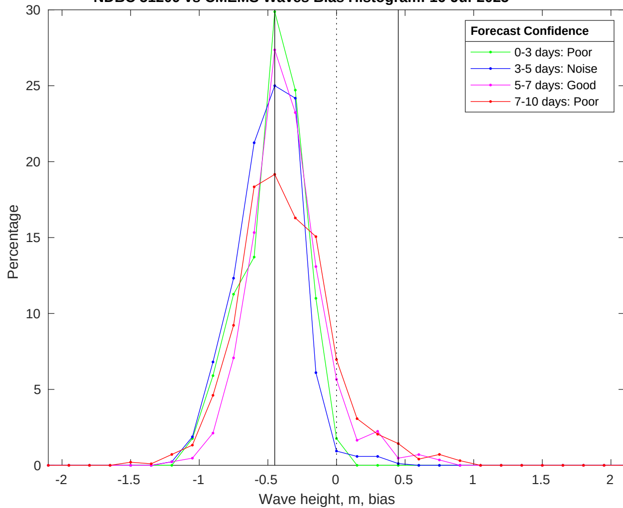
NDBC 51209 vs CMEMS Waves Bias Histogram: 16-Jul-2025
