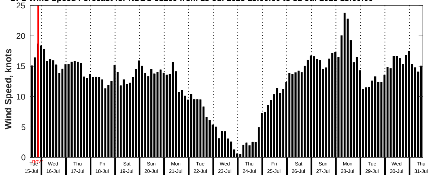
GFS Wind Speed Forecast for NDBC 51209 from 15-Jul-2025 13:00:00 to 31-Jul-2025 13:00:00
