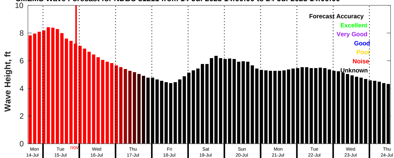
CMEMS Wave Forecast for NDBC 51211 from 14-Jul-2025 14:00:00 to 24-Jul-2025 14:00:00
