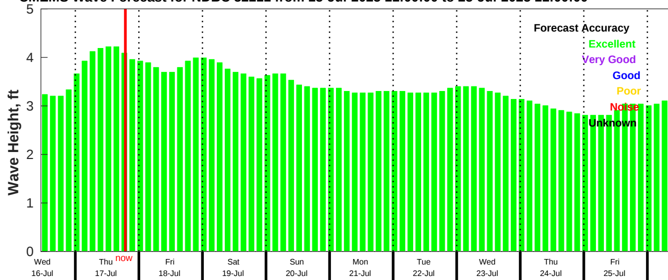
CMEMS Wave Forecast for NDBC 52211 from 15-Jul-2025 11:00:00 to 25-Jul-2025 11:00:00
