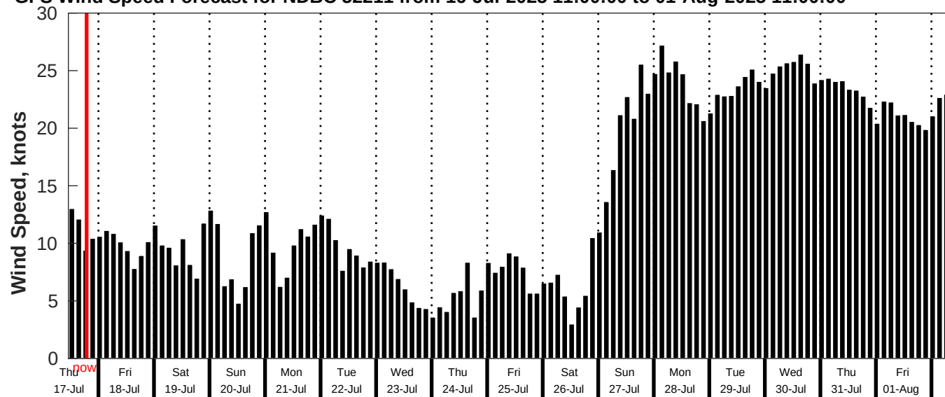
GFS Wind Speed Forecast for NDBC 52211 from 16-Jul-2025 11:00:00 to 01-Aug-2025 11:00:00
