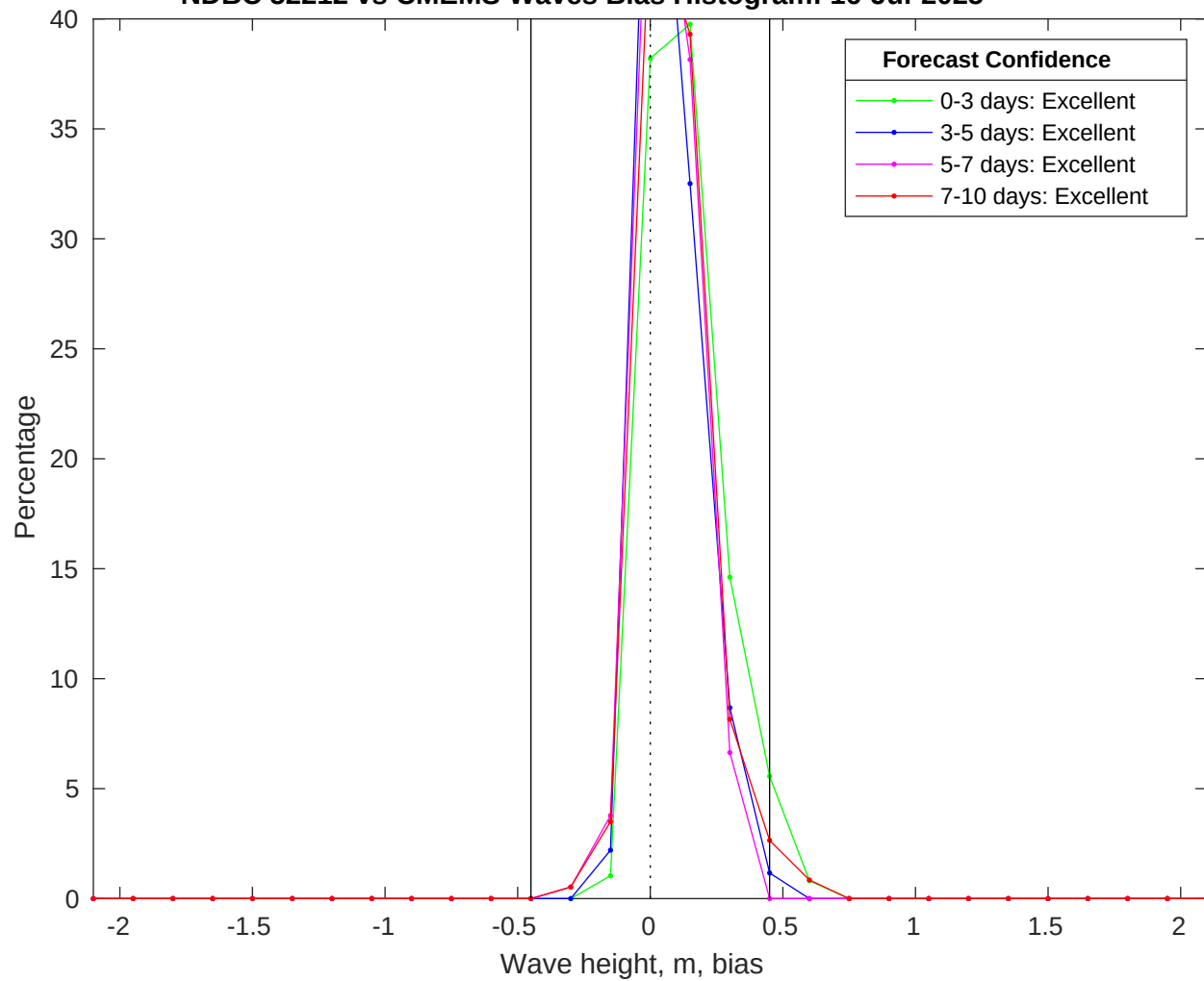
NDBC 52212 vs CMEMS Waves Bias Histogram: 16-Jul-2025
