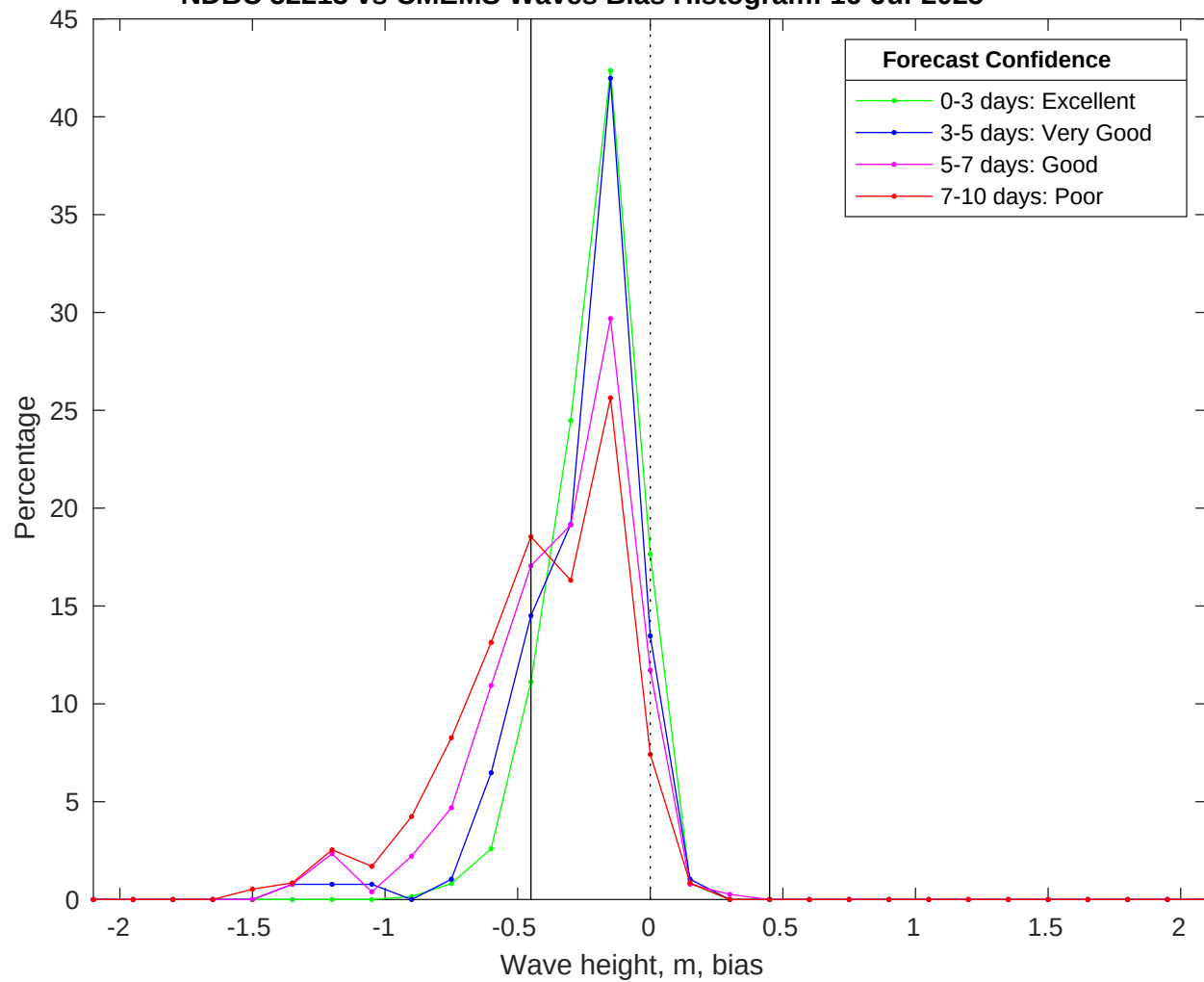
NDBC 52213 vs CMEMS Waves Bias Histogram: 16-Jul-2025
