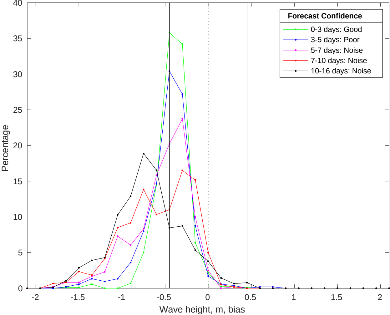
NDBC 52213 vs GFS Waves Bias Histogram: 16-Jul-2025
