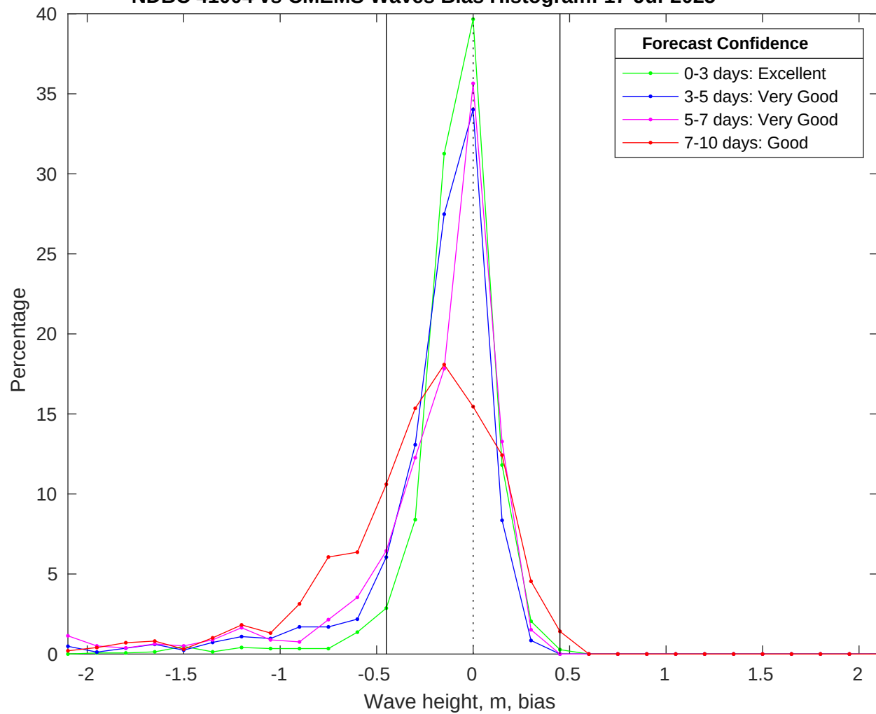
NDBC 41004 vs CMEMS Waves Bias Histogram: 17-Jul-2025
