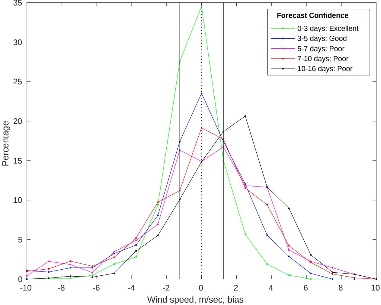
NDBC 41004 vs GFS Winds Bias Histogram: 17-Jul-2025
