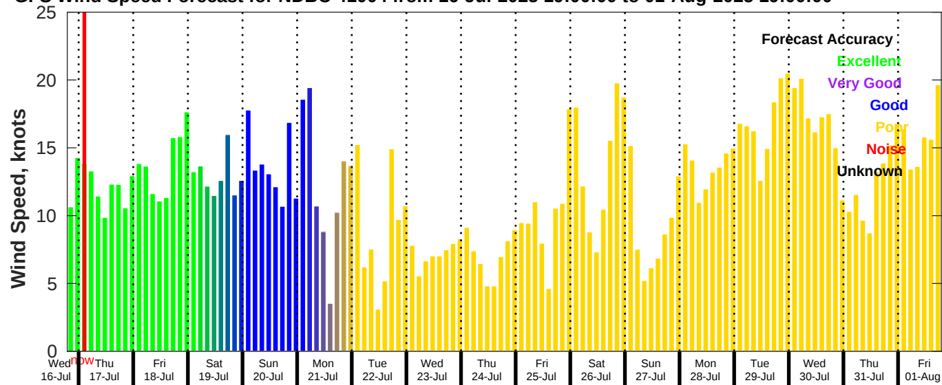
GFS Wind Speed Forecast for NDBC 41004 from 16-Jul-2025 19:00:00 to 01-Aug-2025 19:00:00
