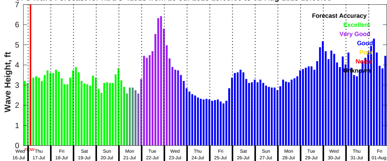
GFS Wave Forecast for NDBC 41013 from 16-Jul-2025 19:00:00 to 01-Aug-2025 19:00:00
