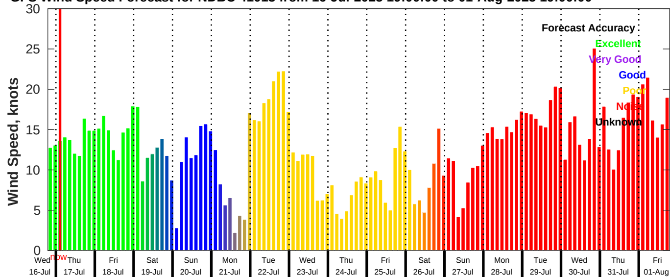
GFS Wind Speed Forecast for NDBC 41013 from 16-Jul-2025 19:00:00 to 01-Aug-2025 19:00:00
