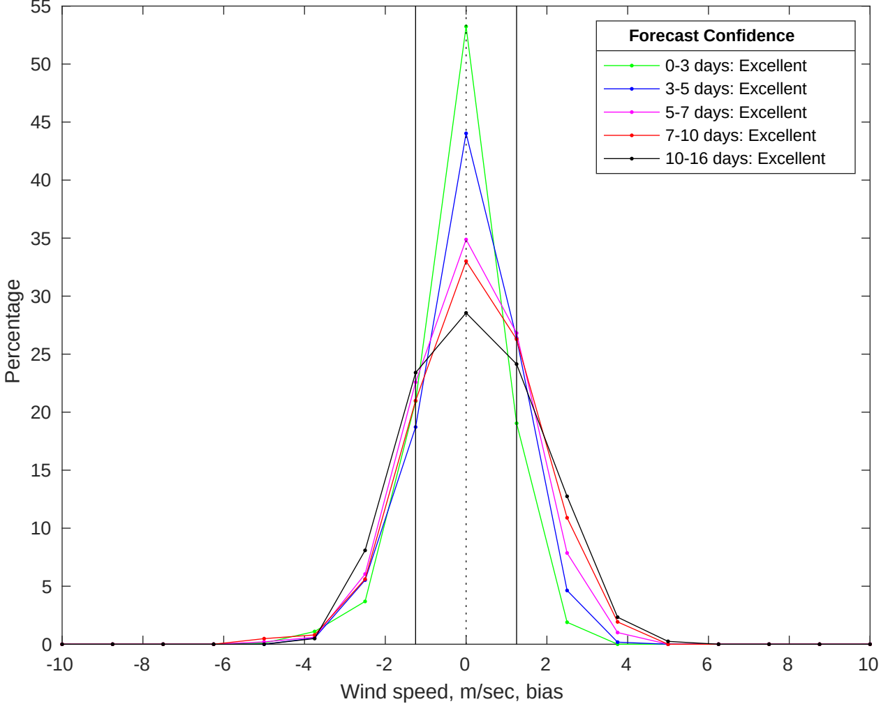
NDBC 41040 vs GFS Winds Bias Histogram: 17-Jul-2025
